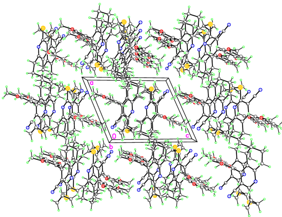
Figure S3. Molecular packing in crystals of compound 1c.
