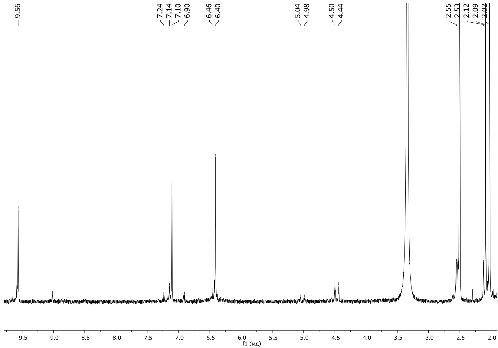
^1\text{H} NMR spectra of the mixture of regioisomeric cage phosphonates 3, 4
